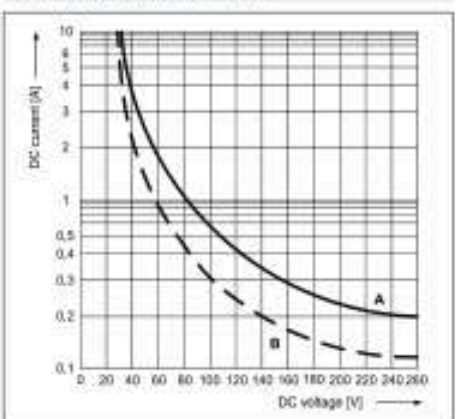
Max. DC breaking capacity Fig. 3.2 A - resistive load DC1 B - inductive load L/R = 40 ms
